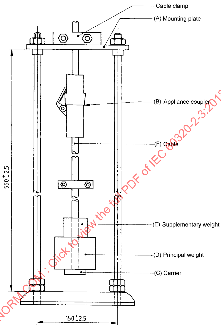
Figure 3 — Example of apparatus for inadvertent disengagement (see 16.101)
