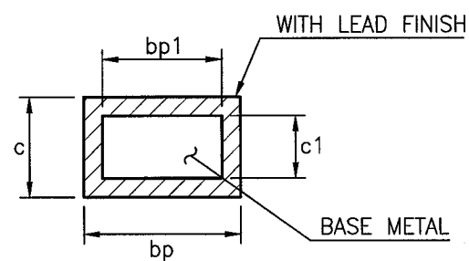
SECTION Z-Z (NOTE 8)
