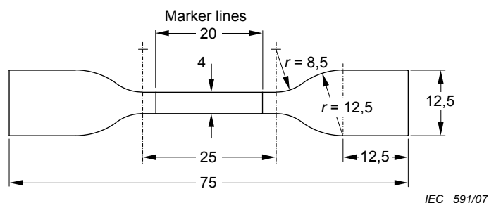
Figure 1 – Dumb-bell test piece
