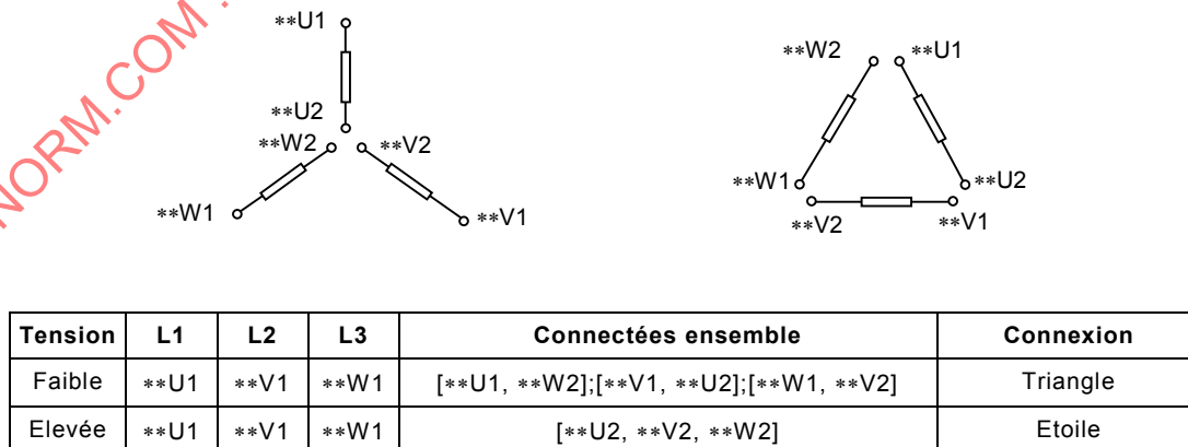
Figure 28 – Triphasé, deux tensions
