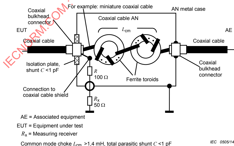
Figure F.1 – Example of a coaxial cable AN
