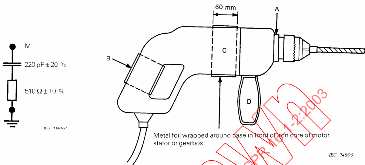
Figure 9a – RC element
