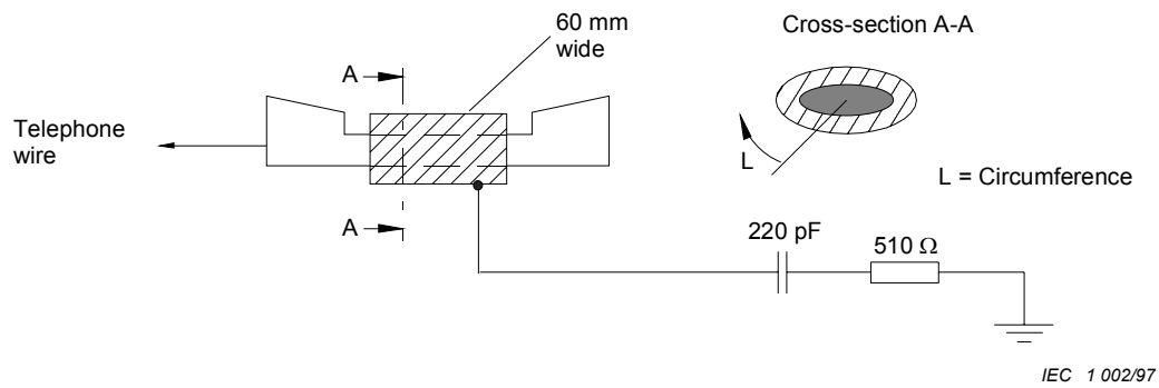
Figure 10a – Application of artificial hand to telephone handset
