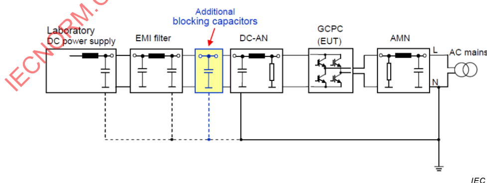
Figure K.3 – Blocking of flow of common mode RF current by employment of additional CM decoupling capacitors
