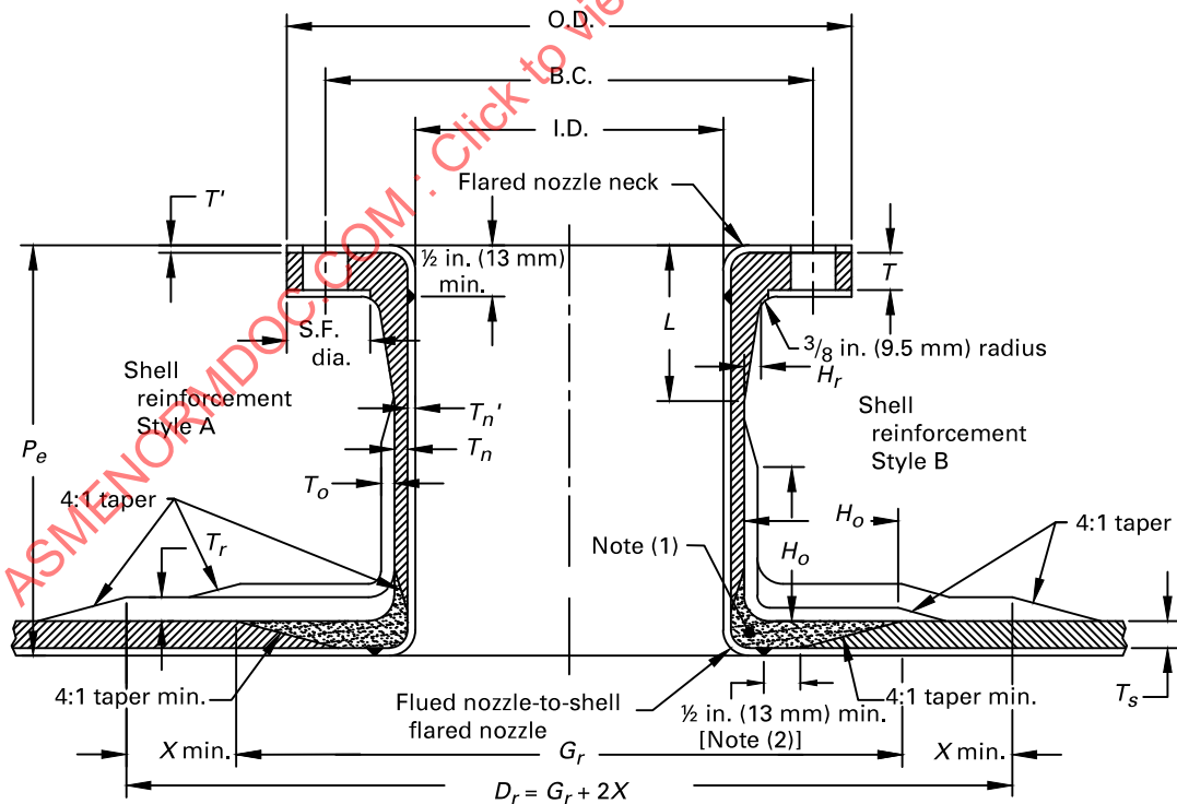
(b) Nozzle Neck Flared
