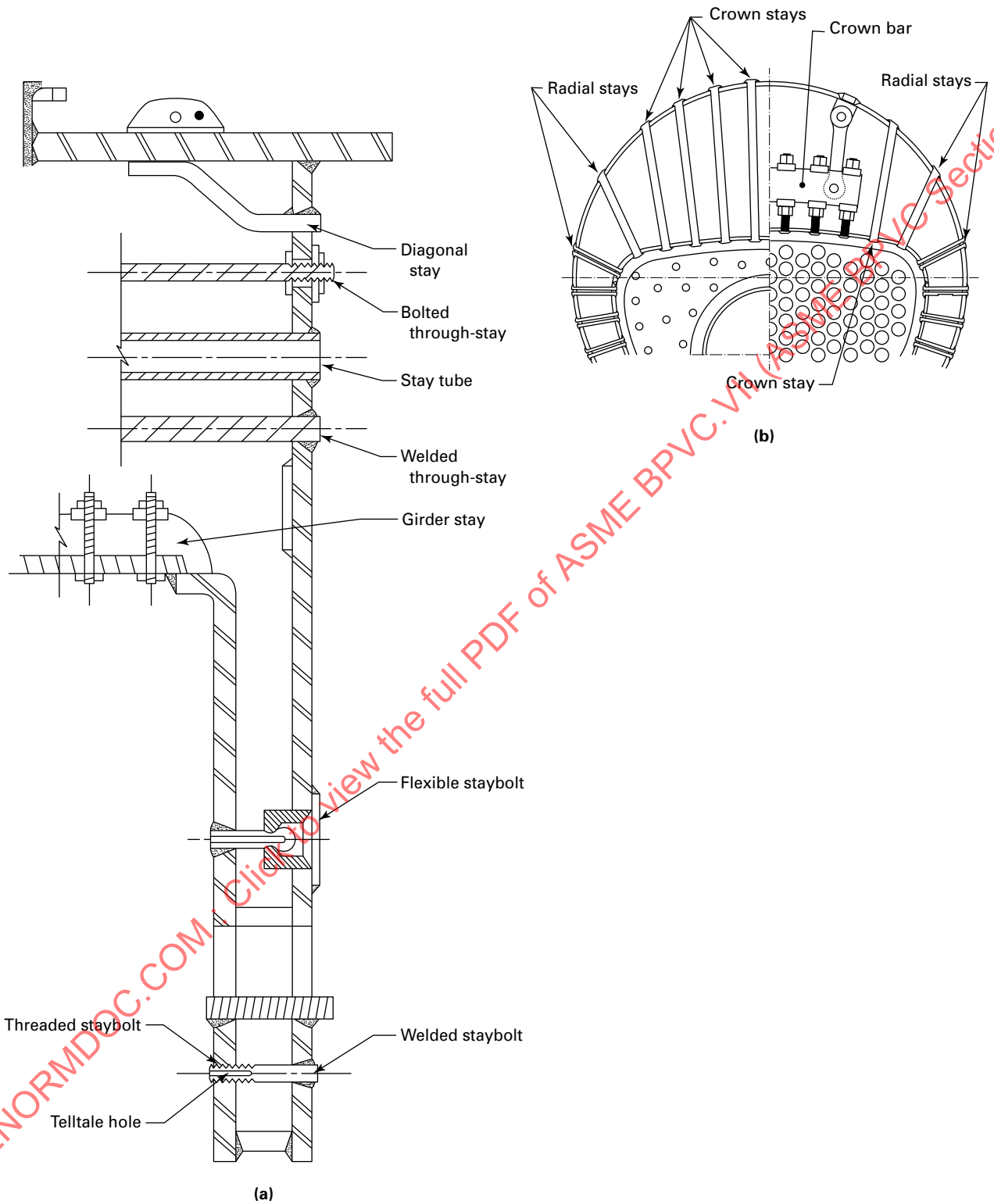
Figure 300.3.1-1 Typical Stays
