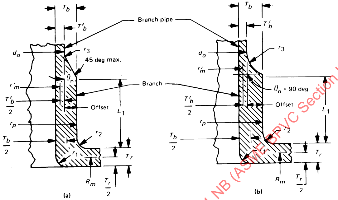
Figure NB-3643.3(a)-1 Branch Connection Nomenclature
