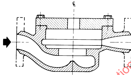
Figure NB-3441.1-2 Type A Pump
