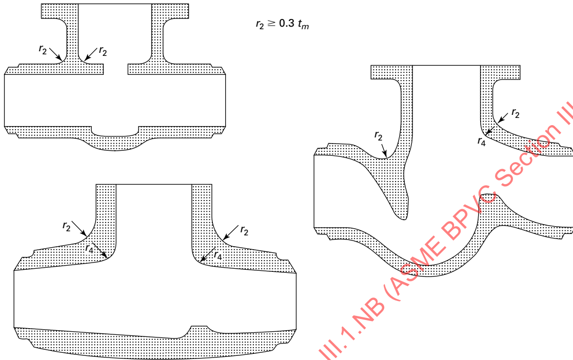
Figure NB-3544.1(a)-1 Fillettes and Corners
