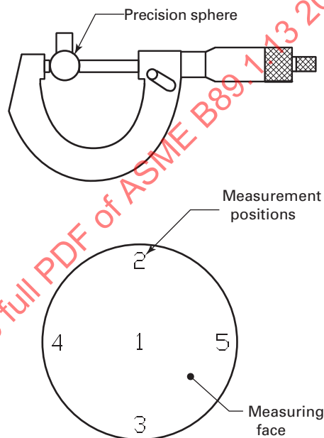
Fig. C-2.4-1 Parallelism Error Test on Small Outside Micrometer
