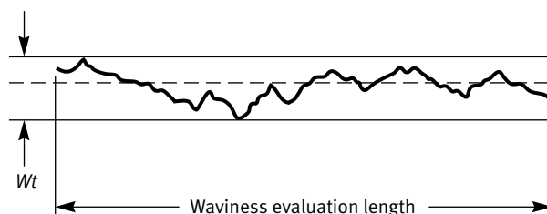
Figure 1-4.1.2-1 The Waviness Height, Wt
