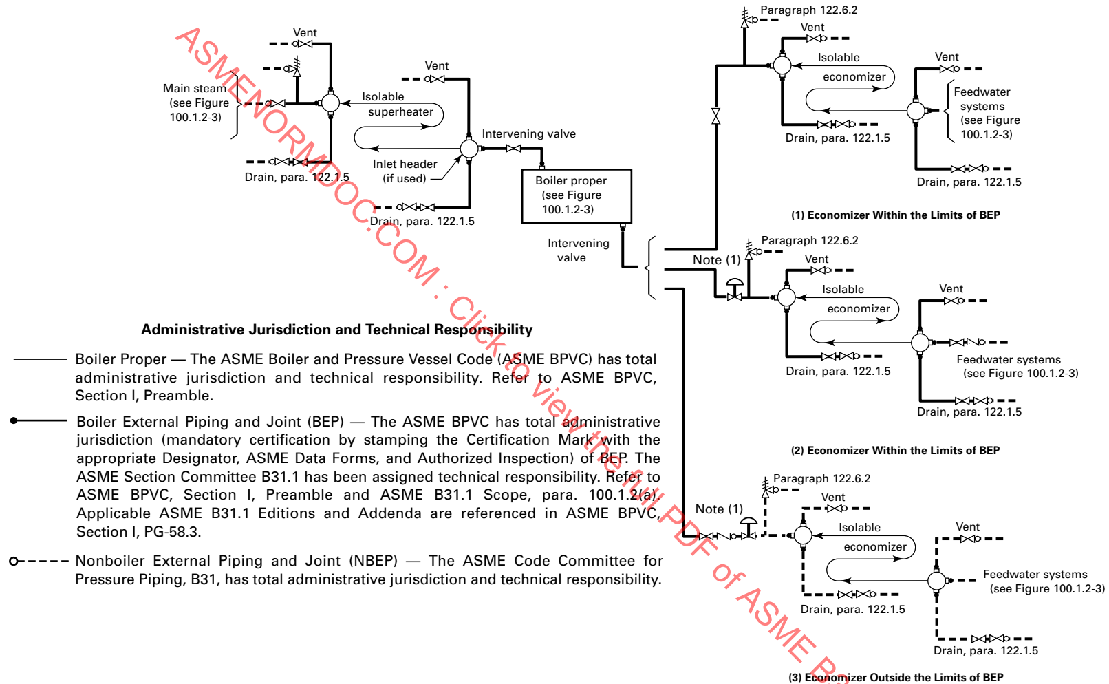
(18) Figure 100.1.2-4 Code Jurisdictional Limits for Piping — Isolable Economizers Located in Feedwater Piping and Isolable Superheaters in Main Steam Piping (Boiler Pressure Relief Valves, Blowoff, and Miscellaneous Piping for Boiler Proper Not Shown for Clarity)
