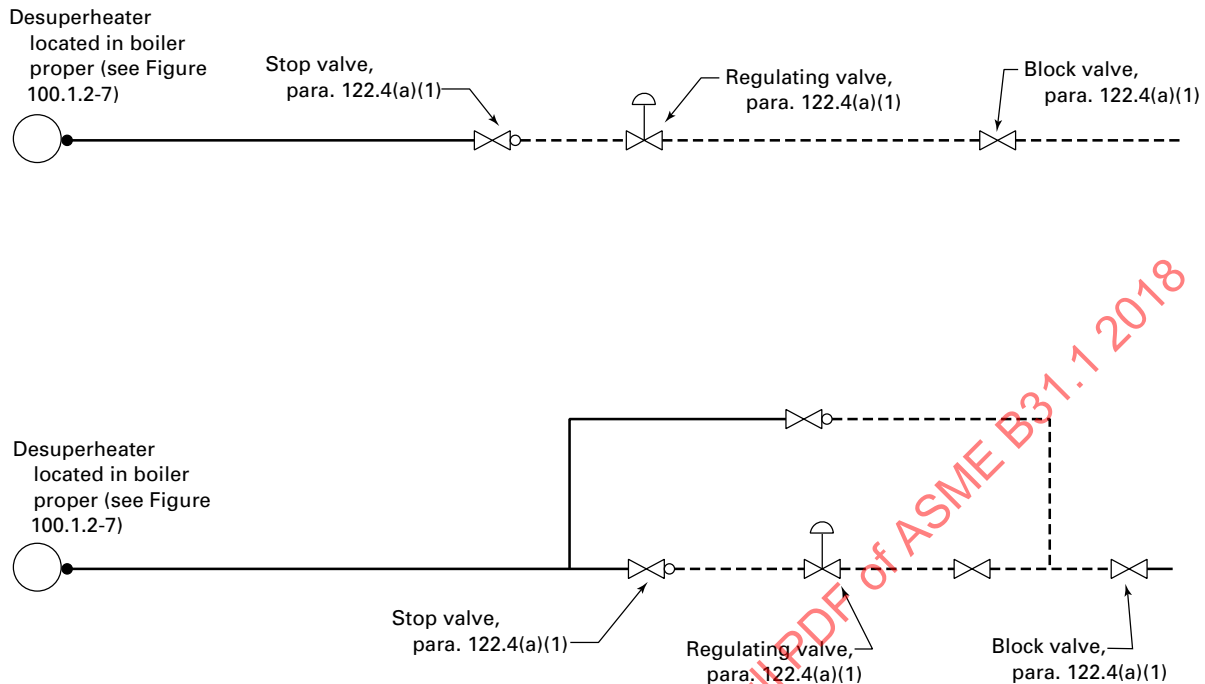
(18) Figure 100.1.2-6 Code Jurisdictional Limits for Piping — Spray-Type Desuperheater
