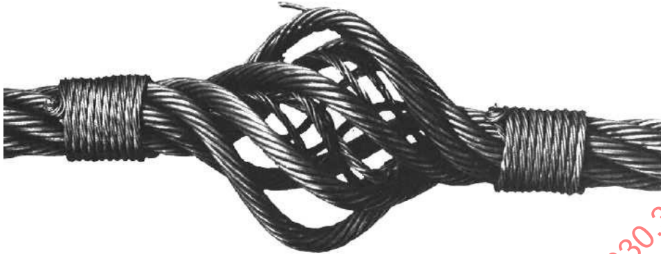
Figure 30-0.2-1 Birdcage Example
