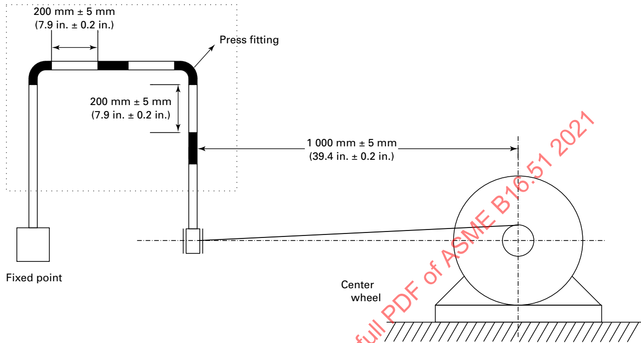
Figure 14.8.1-1 Test Setup for Vibration Test
